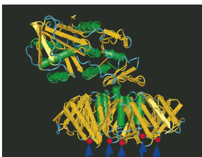
Serine 31 residues of B subunit (x5)
